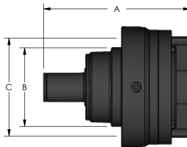
Shaft Output
